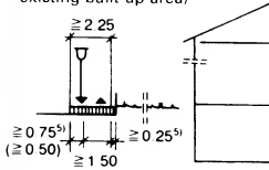
① Footpath running alongside the road
